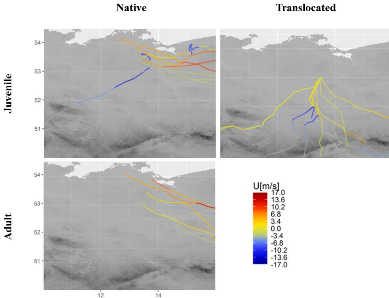
Fig S4. Departure routes of LSEs north of 50°N latitude, with segments colored according to the strength of westward(-)/eastward(+) winds at each preceding GPS-fix (U, see legend). Some eagles departing westward experienced strong westward winds (e.g., blue track top left), but others flew west in relatively light side winds (yellow track, top right). Most eagles departing eastward experienced eastward winds (orange and red tracks top and bottom left), though some experienced weak-moderate westward winds as well (green tracks all graphs).
