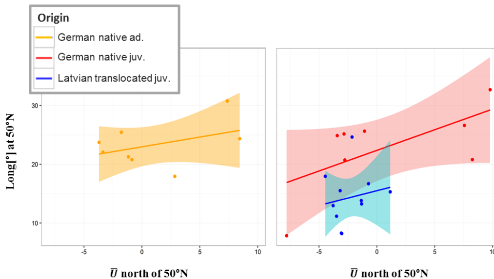
Fig S5. Linear regression models (90% confidence interval) for the longitude at which eagles crossed 50°N latitude, relative to the mean westward(-)/eastward(+) wind strength ( \bar{U} ) encountered north of 50°N. Models were separated according to the birds' age and origin (legend).
